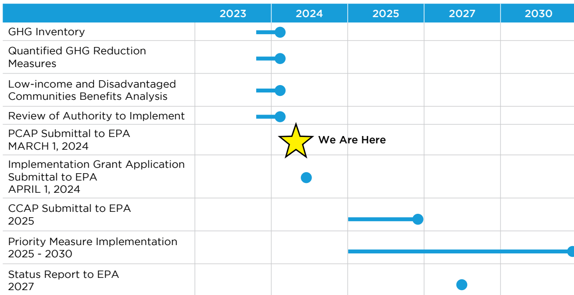
Figure 25: Project timeline
